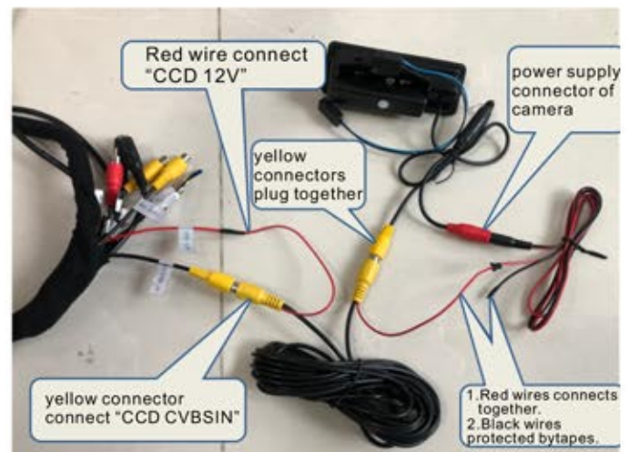
Rear camera wiring for Auto gear.
